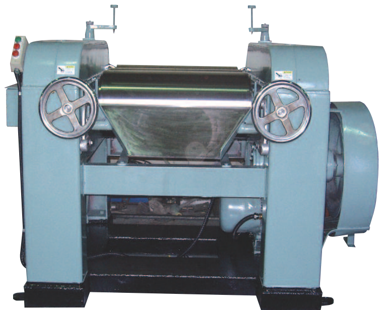
Three-Roll Mill 16"
